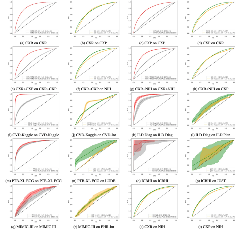
Fig. 1. Cross-hospital classification performance under shortcut shift.
