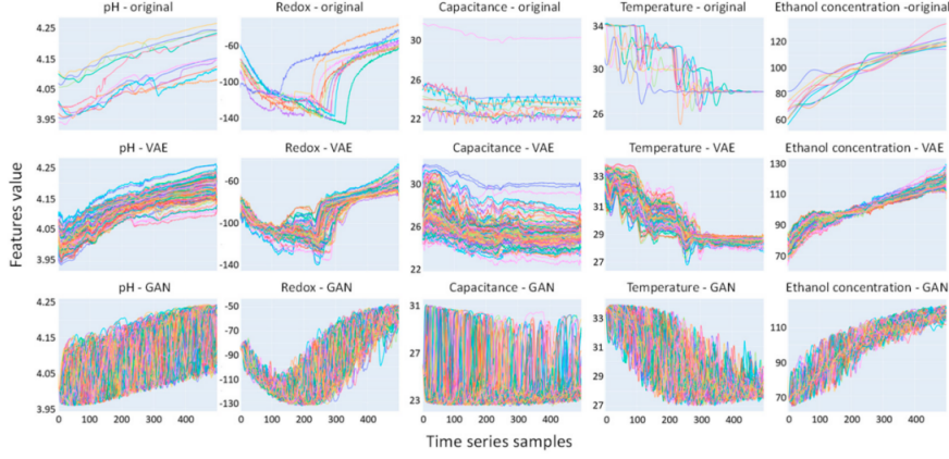
Fig. 1. Time-series changes in fermentation process variables during abnormal events.
